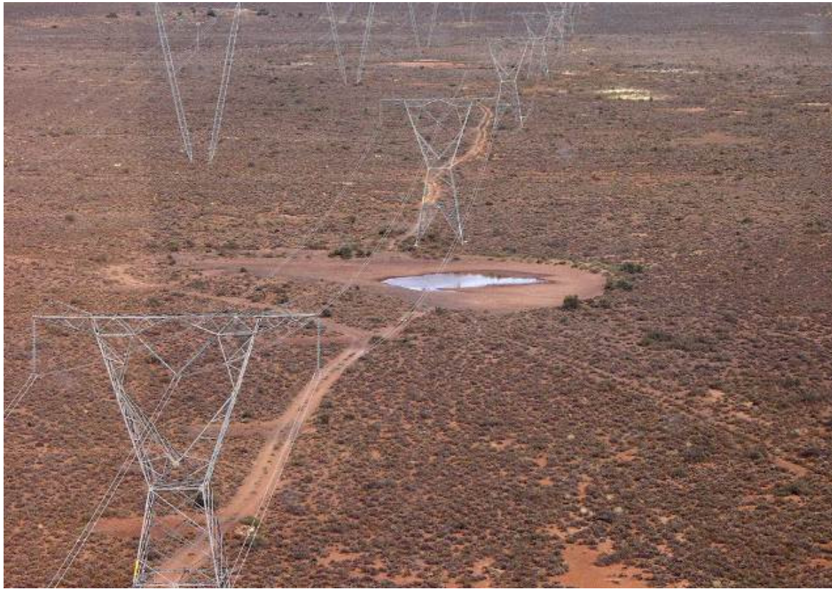
Figure 1. Two adjacent transmission lines in the Karoo region of South Africa. The sum of impacts on birds of two closely spaced lines may be importantly lower than when those lines were positioned far apart (Photo: EWT-WEP).
