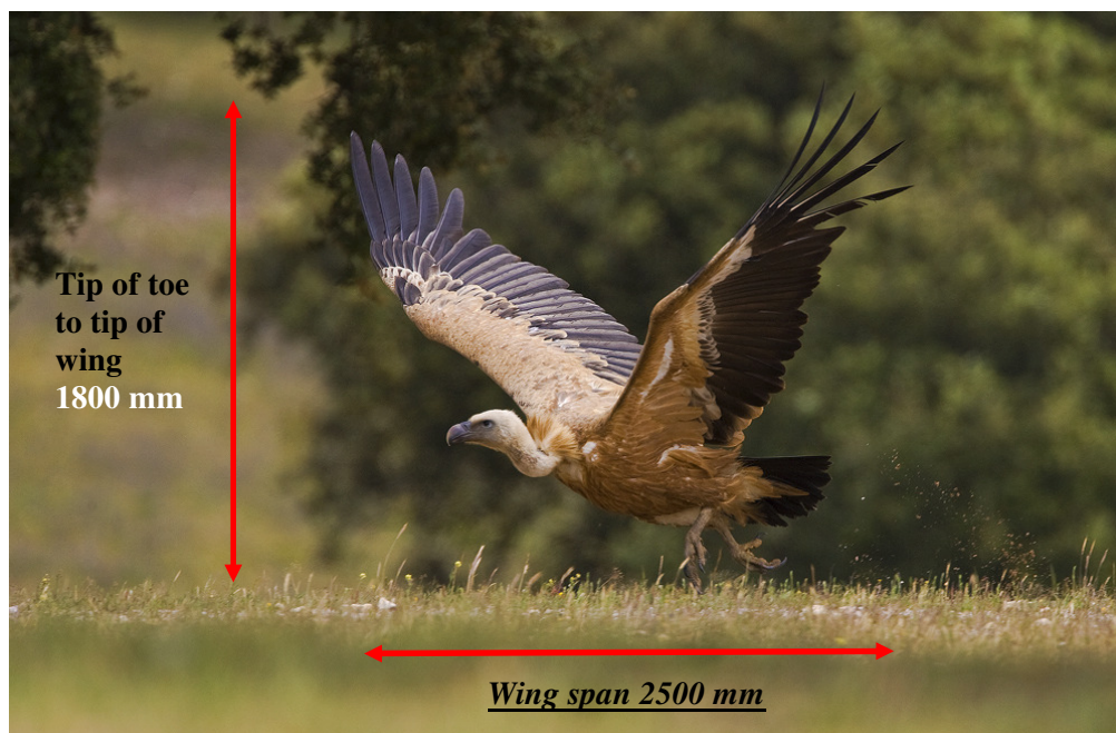
Figure 2. A Griffon Vulture ( Gyps fulvus ) with outstretched wings at take off. To mitigate for bird electrocutation, distances between electric conductors (or phases) and distances between conductors and grounded hardware should be separated over a larger distance than the wrist-to-wrist or head-to-foot distance of a bird. Because dry feathers provide insulation, the distance between fleshy parts, such as skin, feet or bill, is generally the critical factor to determine if a power line construction is safe for perching birds. Note, however, that wet bird feathers provide less insulation, therefore, in wet climates safe distances between energised parts should be based on wingspan and toe-to-wing tip distances of the largest perching protected species in the area (Photo: Bureau Waardenburg).
